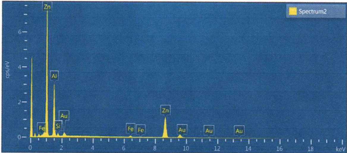
Fig. 4 Spectrum 2 of sample
