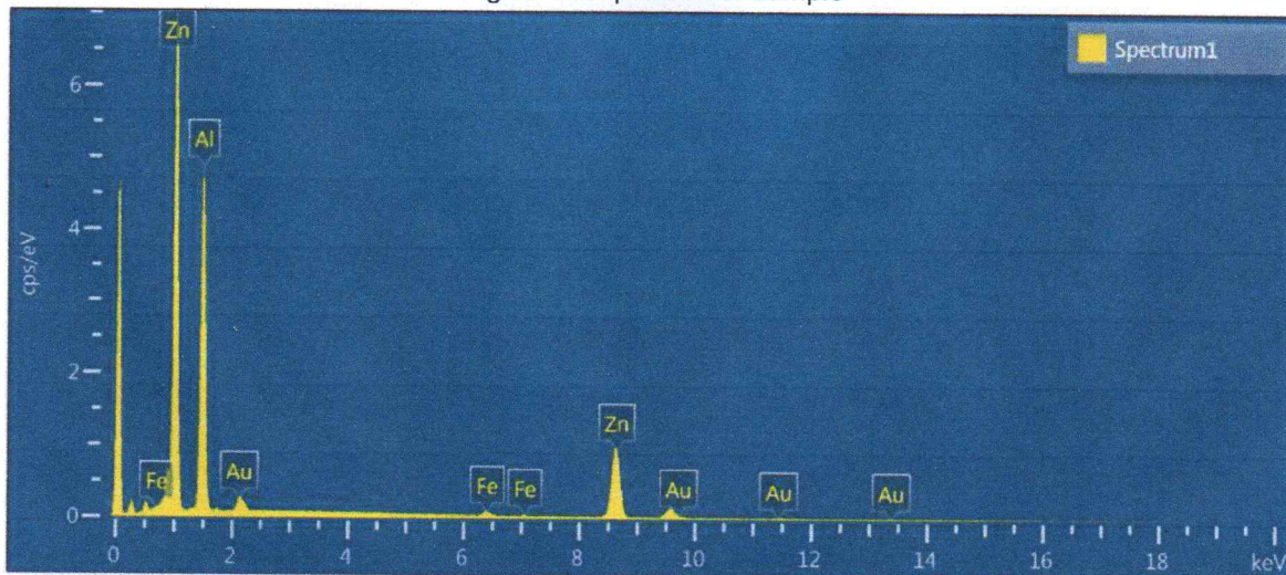
Fig. 3 Spectrum 1 of sample
